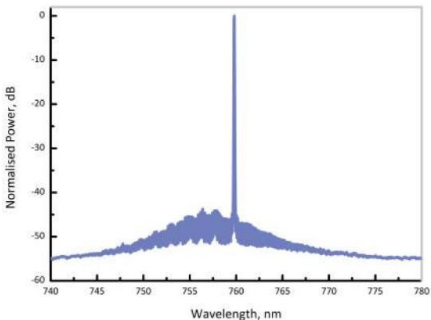
Typical CW Spectrum
