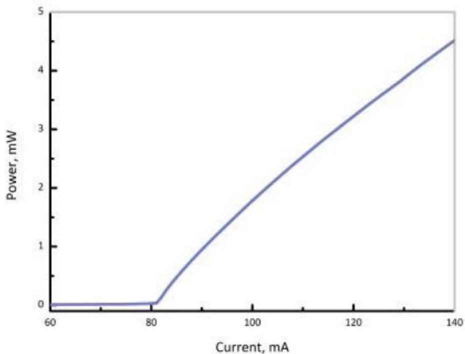
Power vs. Operating Current
